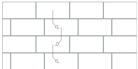
O4BF - Offset 1/4 Back + Forth
